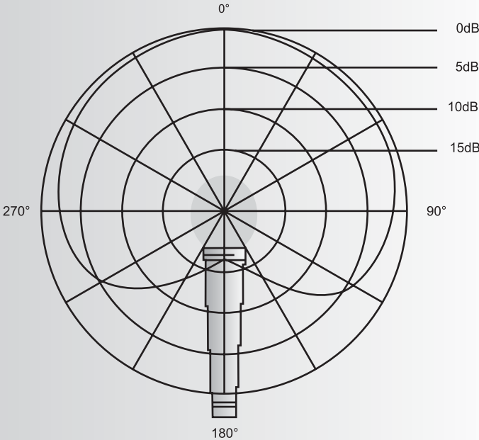
Fig 23. Basic cardioid mic polar pattern
