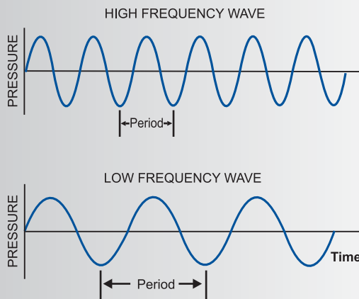
Fig 1-3. Frequency
