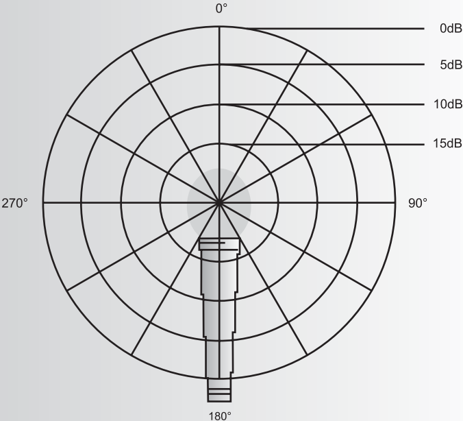
Fig 22. Omnidirectional polar pattern
