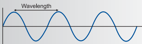
Fig 1-4. Wavelength
