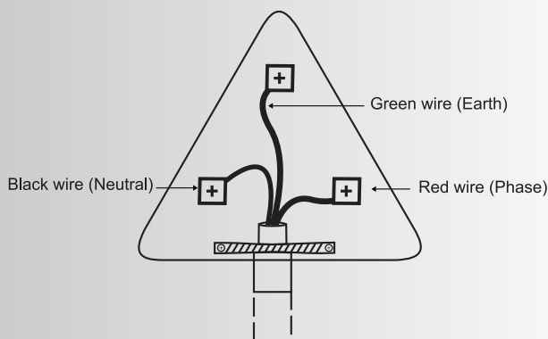
Fig 10: Standard wiring for a 3 pin plug in India.
