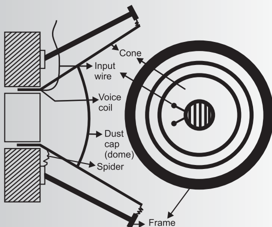
Fig 15. Cross section of a speaker unit
