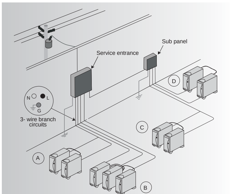
Fig 2-10. Grounding equipment is an important consideration for CR stations. Most modern electronic systems are susceptible to faults caused by poor grounding.
