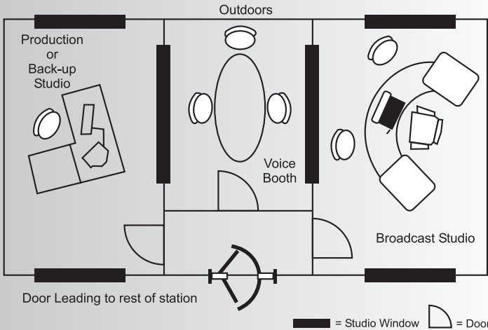
Fig 2-3. Simple three room CR setup
