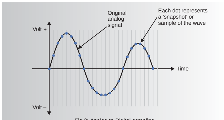
Fig 2: Analog to Digital sampling
