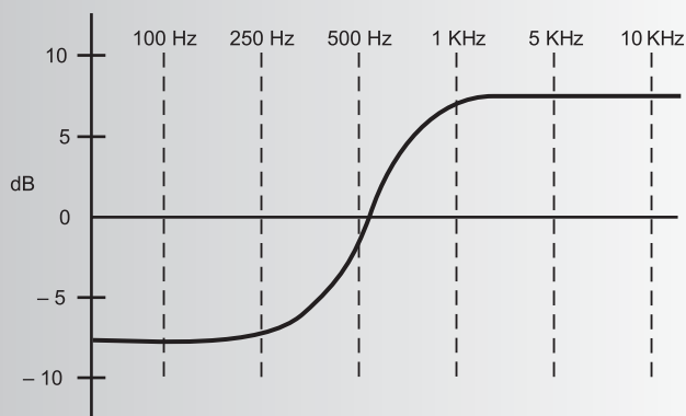
Fig 12. Effect of a low cut/hi pass filter
