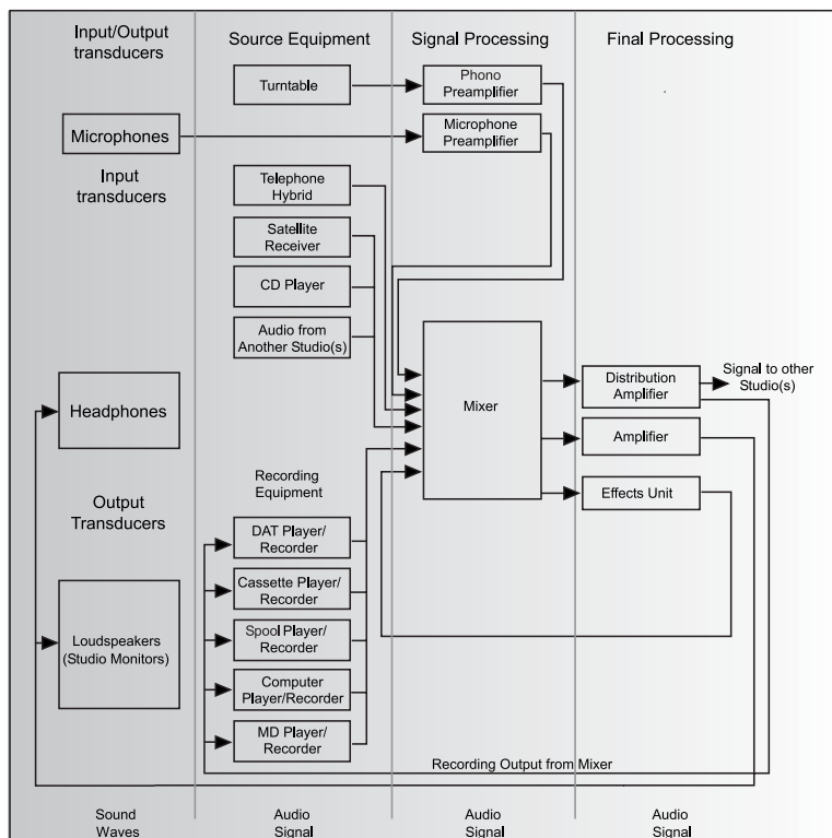
Fig 3-2. Schematic outline of a production studio setup
